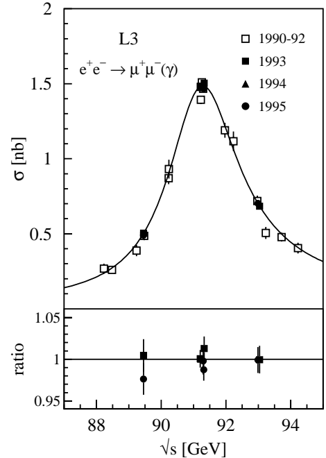
Fig. 25. Same as Fig. 24 for e^+e^- \rightarrow \mu^+\mu^-(\gamma)
